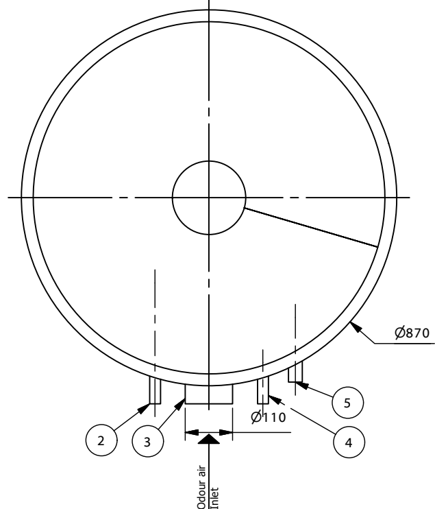
Top View ( 1 : 12 )
